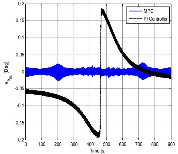
Fig. 8. Elevation angles tracking error
