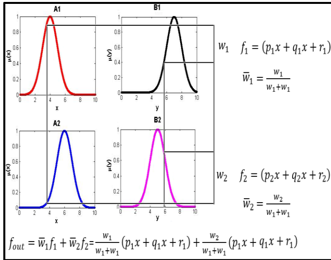
Fig. 1. Inference process of first-order Sugeno.
