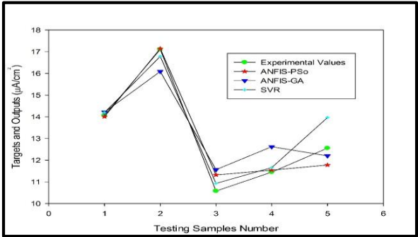
Fig. 8. Comparison between actual and predicted values by ANFIS-PSO, ANFIS-GA, and SVR (testing phase).
