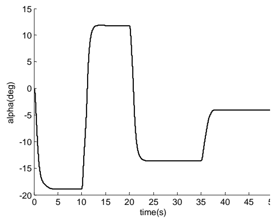
Figure 7. Angle of attack response for Mach 2.3
