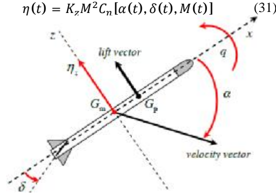
Figure 1. Flying vehicle pitch view
