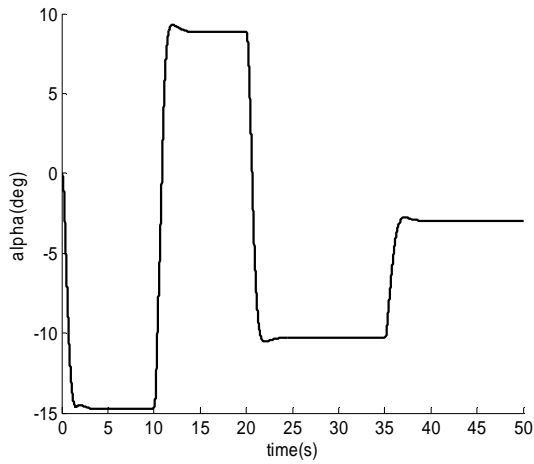
Figure 4. Angle of attack response for Mach 3
