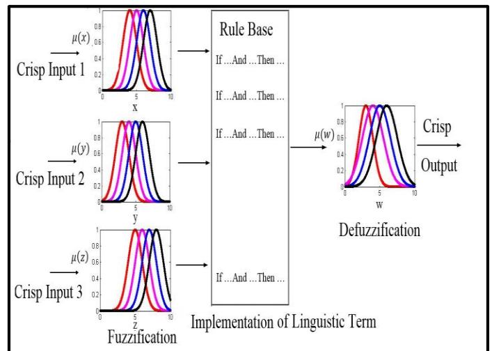
Fig. 3b. Fuzzy inference system diagram.
