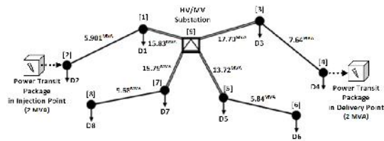
Fig. 7 Optimal network configuration at horizon year for Scenario C.
