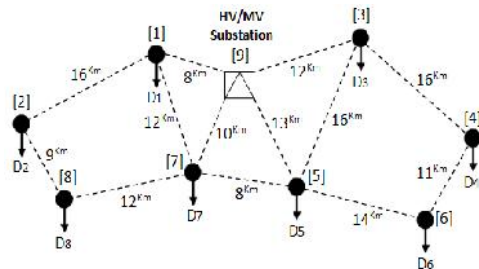
Fig. 4 Primary distribution system under study
