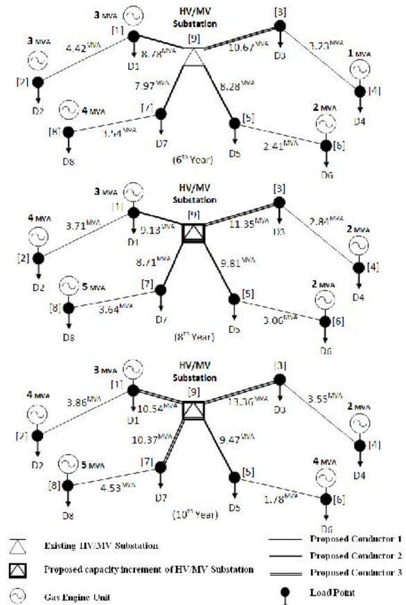
Fig. 6 Proposed radial structure in Scenario-B for each 2-year stage.
