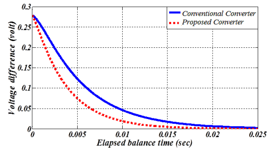
Fig. 8 Comparison between voltages differences versus time
