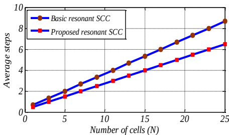
Fig. 6 Average steps for charge transfer in each converter
