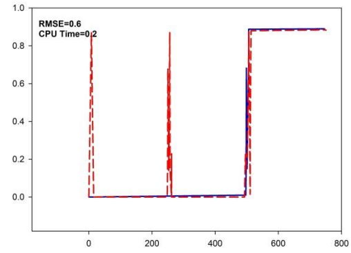
(d) The trained from sEFuNN is tested on the second half of data set
