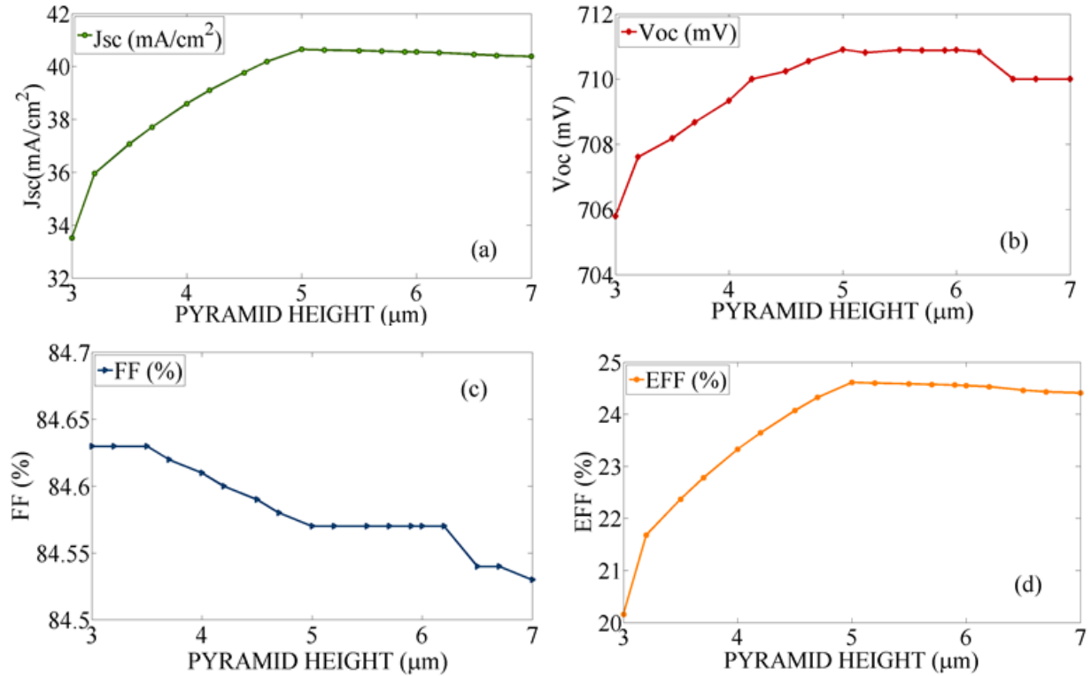
Fig. 3. Solar cell's main parameters as a function of Pyramid height: a) 6 mA increase in J_{SC} , b) 5mV increase in V_{OC} , c) 0.1% reduce in FF and d) more than 4.5% increase in efficiency, resulted due to increase in light absorption by increasing height from 3 to 5\mu m .
