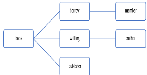
Fig2. Join paths in example library database
