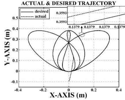
Fig.3. The desired and actual trajectories in Cartesian space for end-effector.
