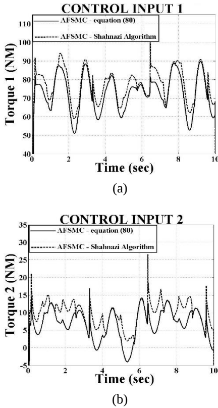
Fig.16. Exerted control inputs to joints 1 and 2, in AFSMC control (equation (80)) compared with AFSMC control (shahnazi algorithm), (a) The exerted control input to joint 1, and (b) The exerted control input to joint 2.
