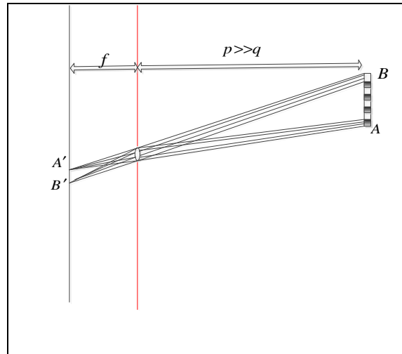
Figure 1. image formation for an object in infinitive using a lens
