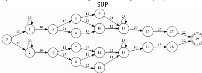
Fig. 13. The feasible supervisor for the guide way \Sigma_{uo} = \{13, 23\} , SUP
