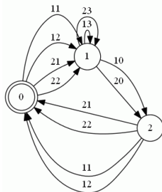
Fig. 13. The feasible supervisor for the guide way \Sigma_{uo} = \{13, 23\} , SUP
