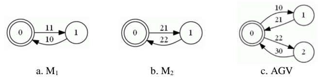
Fig. 15. DES model of each machine and AGV
