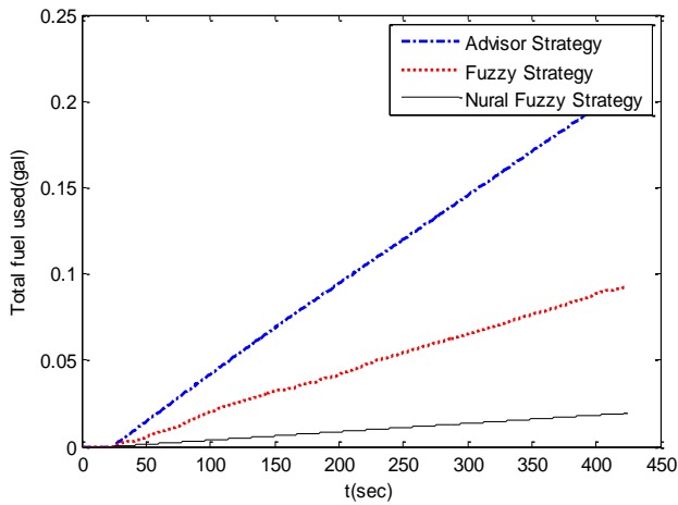
Fig.20. Controller effect on fuel consumption
