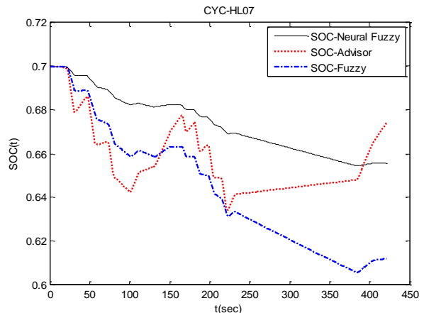
Fig. 24. Controller effect on SOC
