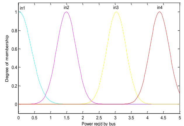
Fig 12. First input of FLC, P1
