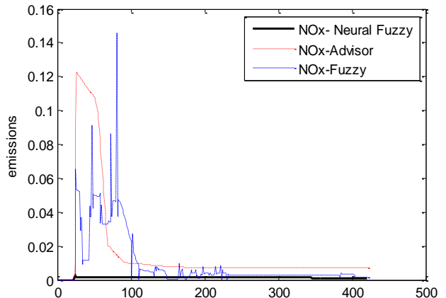
Fig23. Controller effect on NOx pollutant emission
